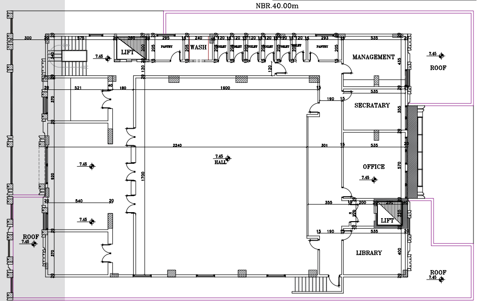
1 FIRST FLOOR PLAN AR-03 SCALE 1:100
